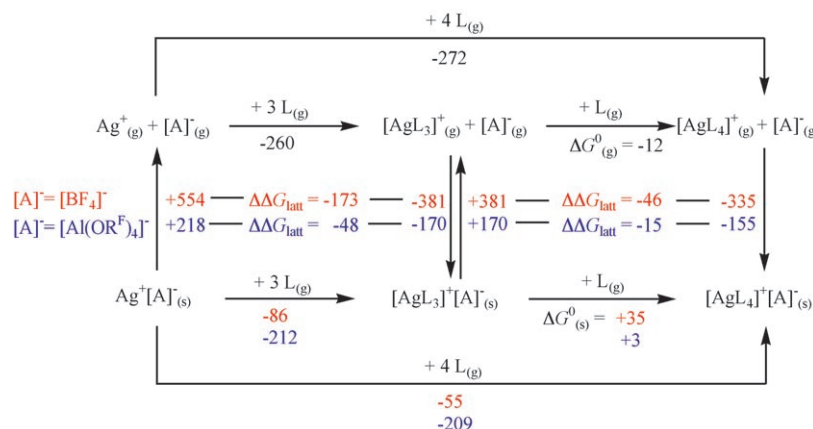
Figure 1. Born-Haber cycle with \Delta G^0 values [ \text{kJ mol}^{-1} ] at 298.15 K. Gas-phase reaction energy calculated at MP2(FC)/TZVPP, thermal and entropic corrections at the BP86/SV(P) level (ref. [19]). For solid-state reactions and lattice energies, upper values (red) count for [\text{A}]^- = [\text{BF}_4]^- , lower values (blue) for [\text{Al}(\text{OC}(\text{CF}_3)_3)_4]^- .
